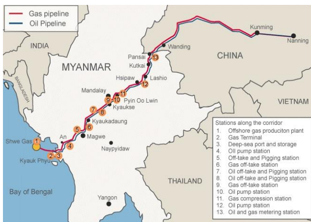
Figure 2: Myanmar-China oil and Gas Pipeline [21]
